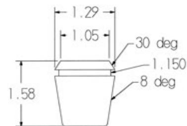
ER32 Collet Dimensions.
