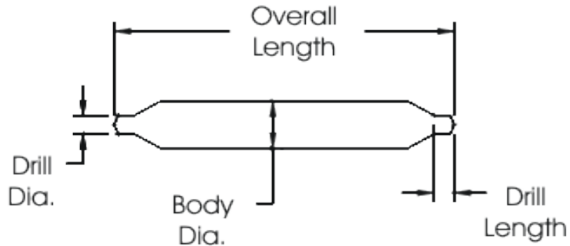
Center Drill Chart
